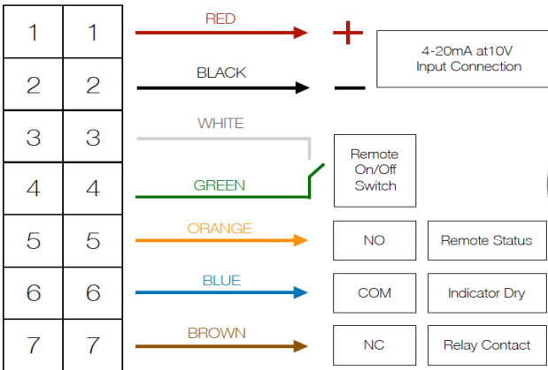
Standard Remote Control Schematic
